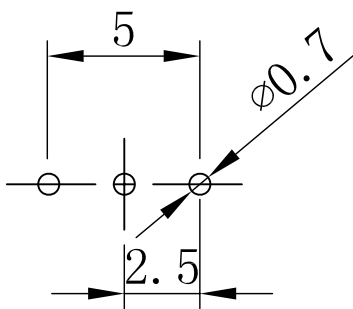
Mounting hole detail
